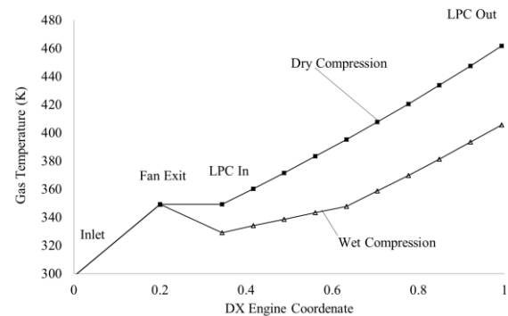
Figure 1. Gas Temperature vs x Coordinate. Comparison between dry and wet compression cases.
